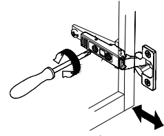
Depth adjustment
